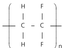
Figure A.1: Chemical structure of PVDF-UHP.
