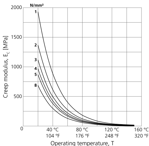
Figure A.13: Creep modulus of ECTFE for 10 year.
