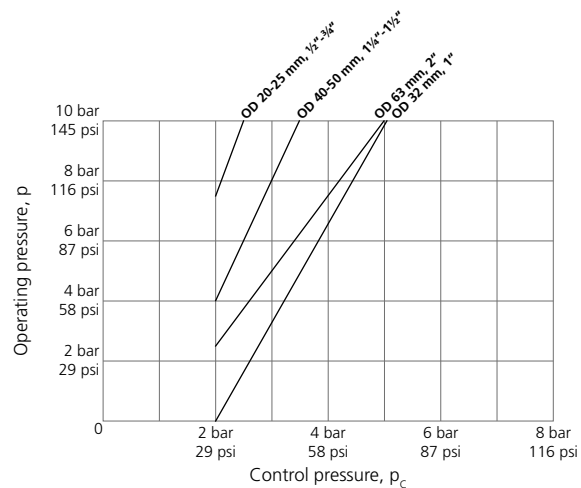
Figure G.28: DA control pressure for EPDM diaphragms.
