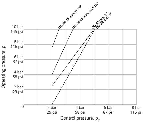
Figure G.41: DA control pressure for EPDM diaphragms.
