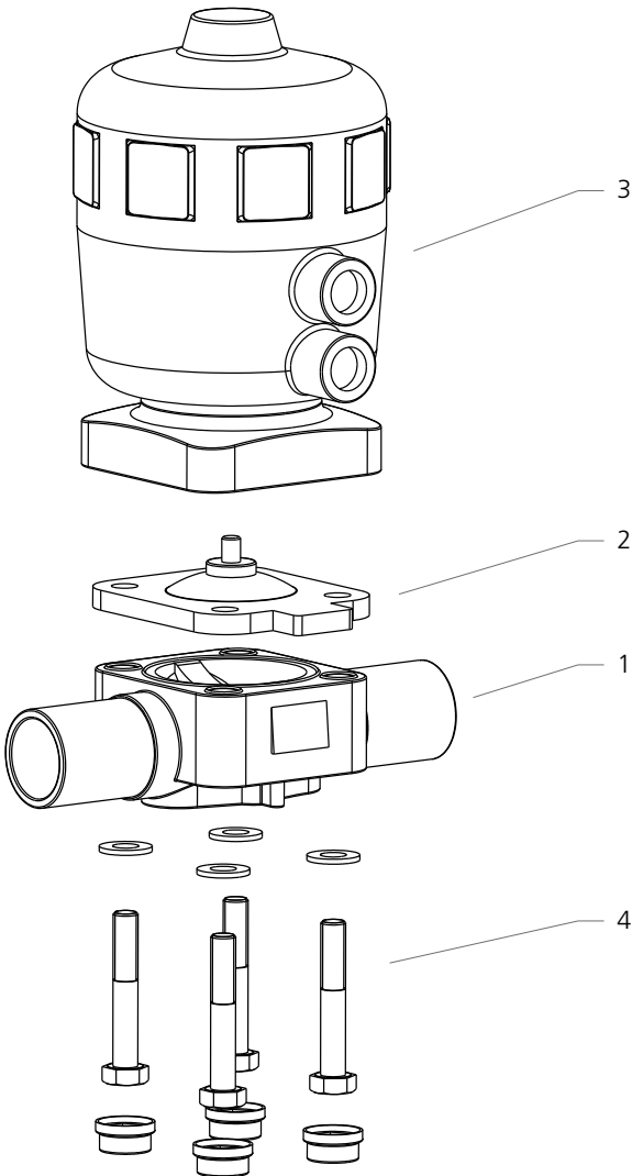
Figure G.21: Exploded assembly drawing.
