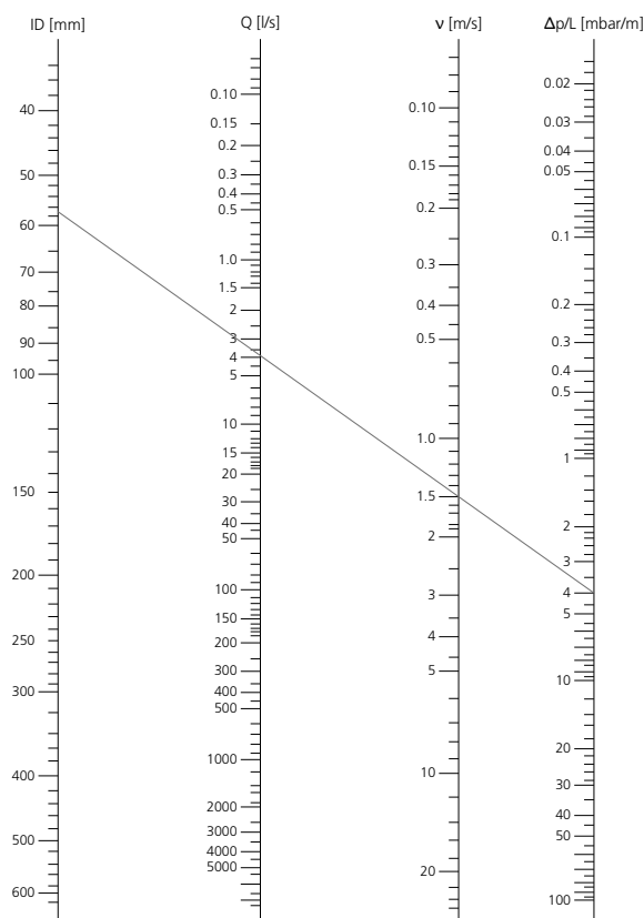
Figure D.5: Flow nomogram example.
