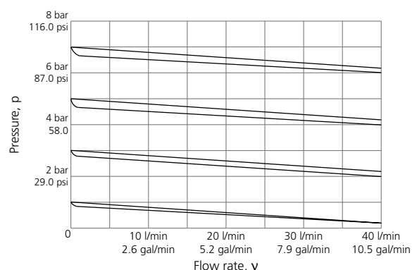
Figure G.72: Characteristic diagram for DN 20 (OD 25 mm, OD 3/4").
