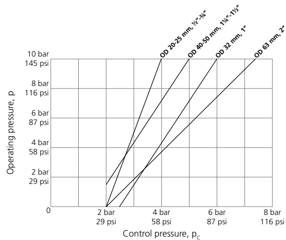
Figure G.27: NO control pressure for EPDM/PTFE diaphragms.
