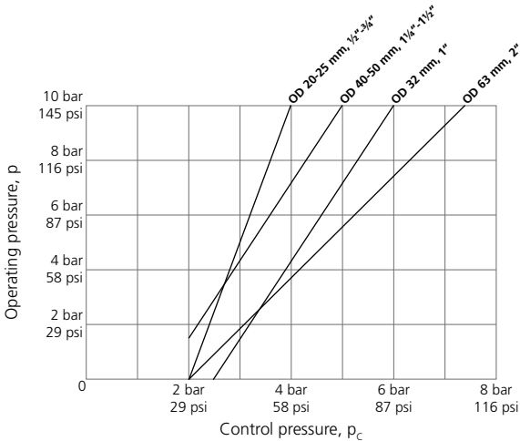
Figure G.40: NO control pressure for EPDM/PTFE diaphragms.
