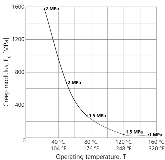
Figure A.11: Creep modulus of ECTFE (100h).
