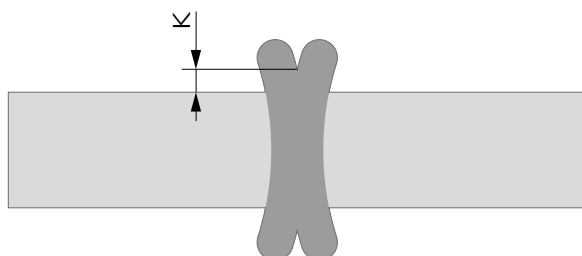
Figure F.13: Bead height K .
