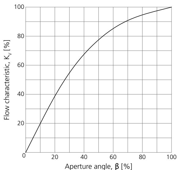
Figure G.22: Flow characteristic.
