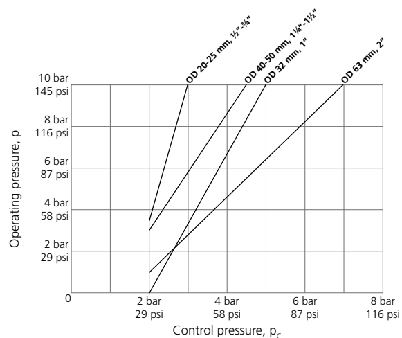
Figure G.29: DA control pressure for EPDM/PTFE diaphragms.
