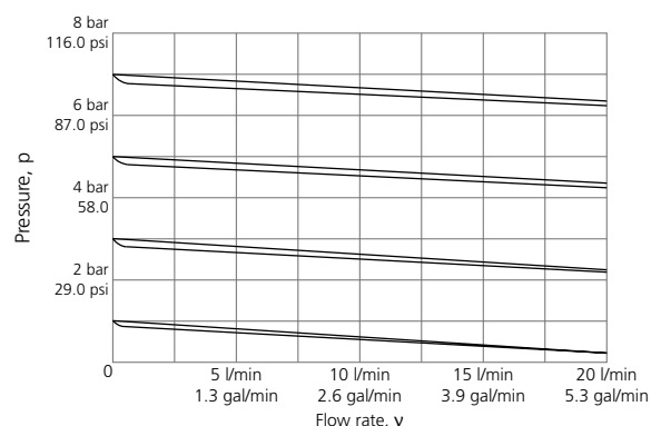
Figure G.71: Characteristic diagram for DN 15 (OD 20 mm, OD 1/2").
