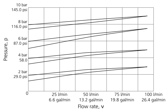
Figure G.89: Characteristic diagram for DN 32 (OD 40 mm, OD 1¼").
