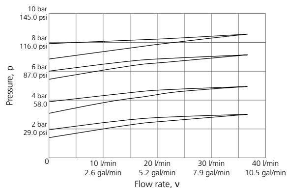
Figure G.87: Characteristic diagram for DN 20 (OD 25 mm, OD ¾").
