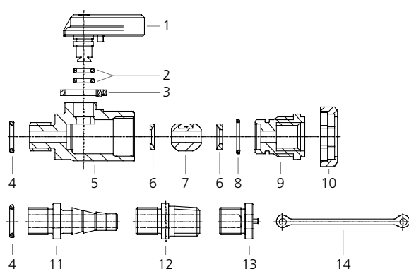
Figure G.8: Exploded assembly drawing.
