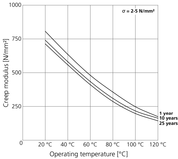
Figure A.3: Creep modulus curves of PVDF-UHP.
