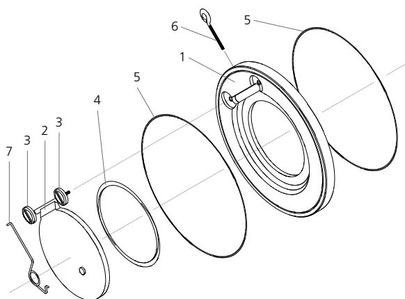
Figure G.53: Exploded assembly drawing.
