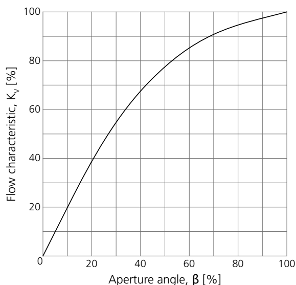
Figure G.14: Flow characteristic.
