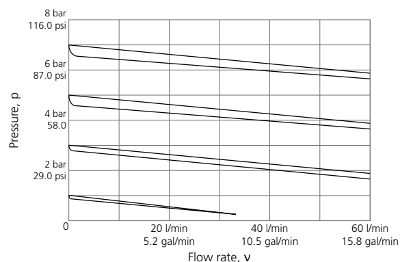
Figure G.73: Characteristic diagram for DN 25 (OD 32 mm, OD 1").
