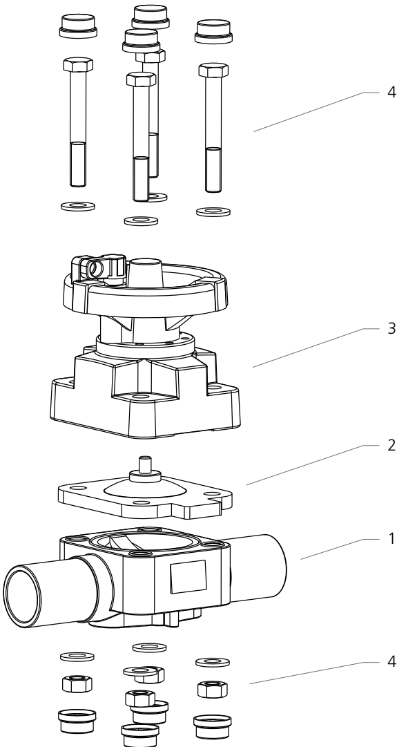
Figure G.13: Exploded assembly drawing.
