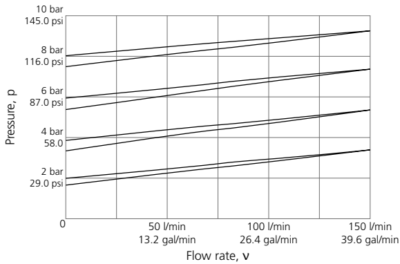
Figure G.90: Characteristic diagram for DN 40 (OD 50 mm, OD 1 1/2").
