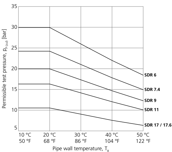
Figure F.22: Test pressure curves for piping made of PP-Pure and Polypure (PP-R).
