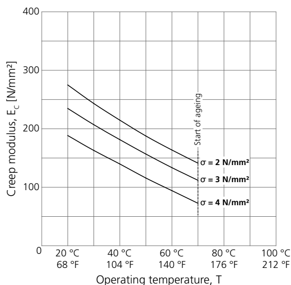
Figure A.8: Creep modulus of PP-Pure and Polypure for 25 years.
