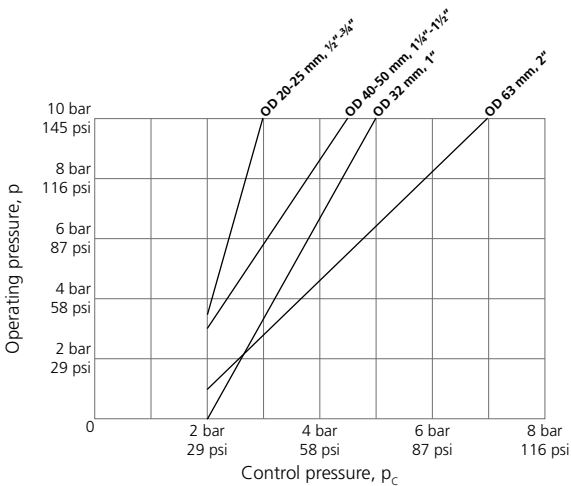
Figure G.42: DA control pressure for EPDM/PTFE diaphragms.
