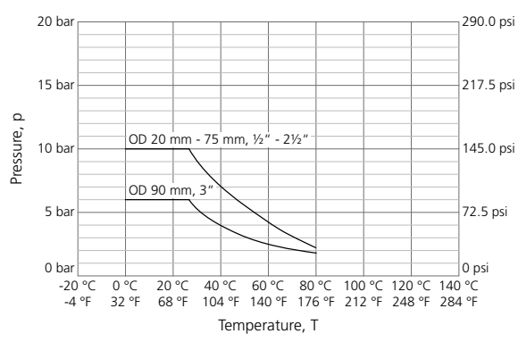
Figure G.6: Pressure - temperature - diagram of PP-Pure valid for water and a service life of 25 years.
