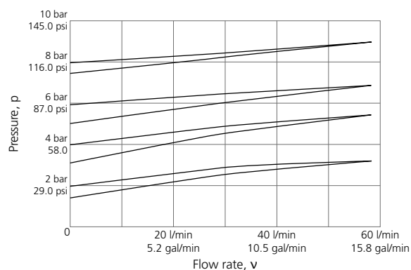
Figure G.88: Characteristic diagram for DN 25 (OD 32 mm, OD 1").
