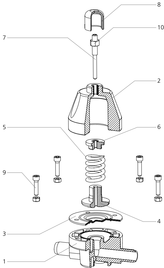
Figure G.77: Exploded assembly drawing.
